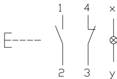
13 Illuminated pushbutton actuator double page 8
